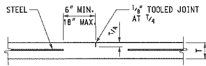
CONTRACTION JOINT
