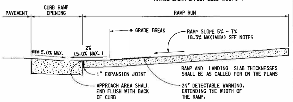
SIDEWALK RAMP PERPENDICULAR TO TANGENT CURB (TYPE F AND TYPE RF SHOWN)
